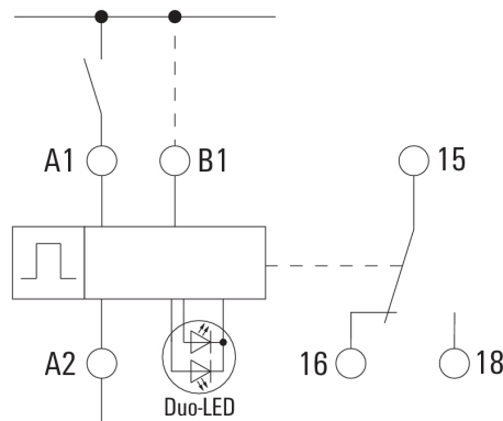
Wiring example
